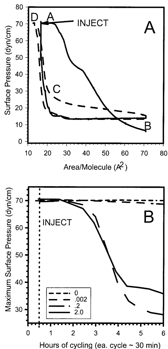
FIGURE 2 ( A ) Isotherms and ( B ) maximum surface pressure vs. elapsed time for the model RLS composed of 69 w/w% DPPC, 21 w/w % POPG, 10 w/w% PA on a 25°C buffered subphase before and after injection of BSA. ( A ) The first cycle is denoted by the solid line, the second (postinjection) by the dotted line. The cycles show no overlap of the collapse plateau (points A, D), indicating that no material returns to the interface during the expansion of the interface after injection of albumin. The lowest surface pressure obtained at maximum trough expansion increases from 0 without albumin (Fig. 1) to >14 dyn/cm ( B ). ( B ) Surface pressure at minimum trough area for the RLS monolayer for 6 h after injection; subphase albumin concentrations range from 0 to 2 mg/ml. Speed of area dilation was 0.096 \text{ cm}^2/\text{s} for all cycles; each cycle took \sim 30 min. Note that all concentrations require at least 2–3 h to significantly lower maximum surface pressure. Because the impact is also not proportional to albumin concentration (0.2 and 2 mg/ml show the same effect), it is clear that solubilization is not important.
