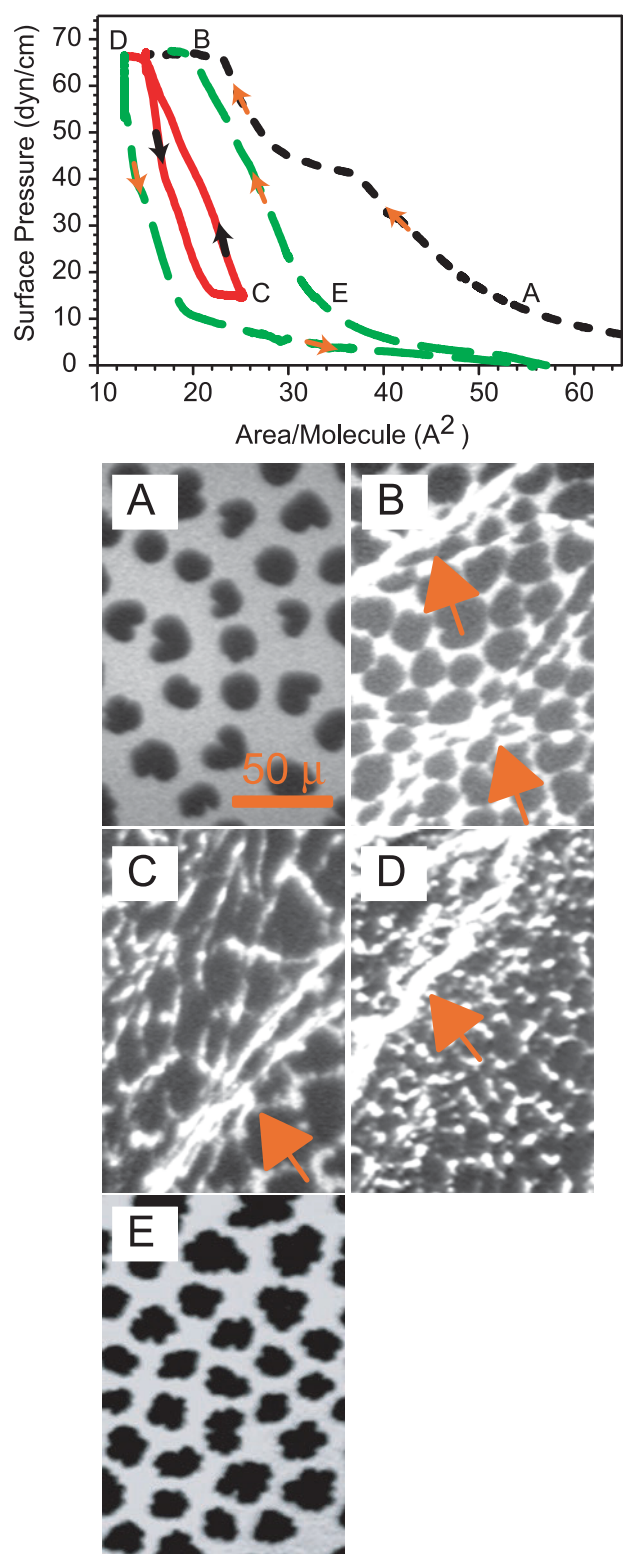
FIGURE 4 Successive isotherms and fluorescence micrographs for the model RLS on a 25°C buffered subphase. The monolayer is first compressed to collapse (black dotted line); however, in contrast to Fig. 1, the expansion is controlled so that surface pressure drops back to 15 dyn/cm and maintained at that pressure for 20 min before recompression to the same collapse pressure (red line). The monolayer is then fully expanded to a surface pressure of zero and again compressed to collapse (green dotted
